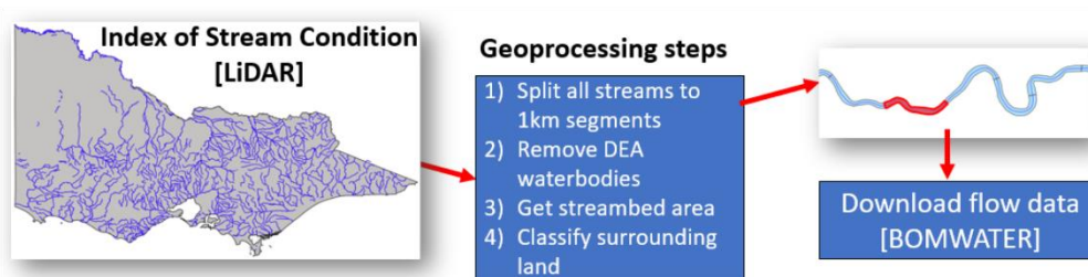
Figure 1. Overview of the waterbody (A) and river/stream (B) GIS layers and processing steps used to estimate the number of waterbodies, rivers and streams with surface water in Victoria.
